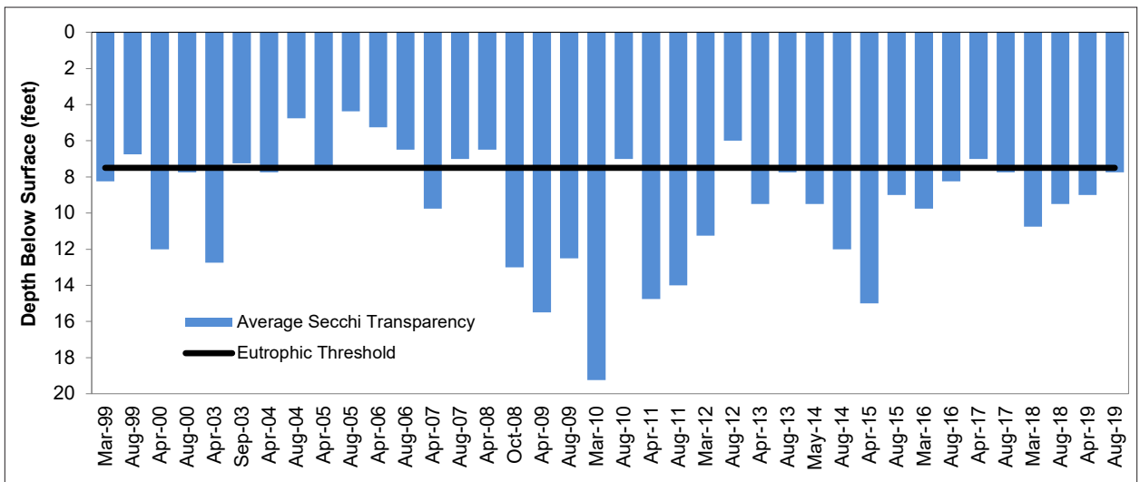
Figure 9. Average Secchi transparency measurements, 1999-2019.
