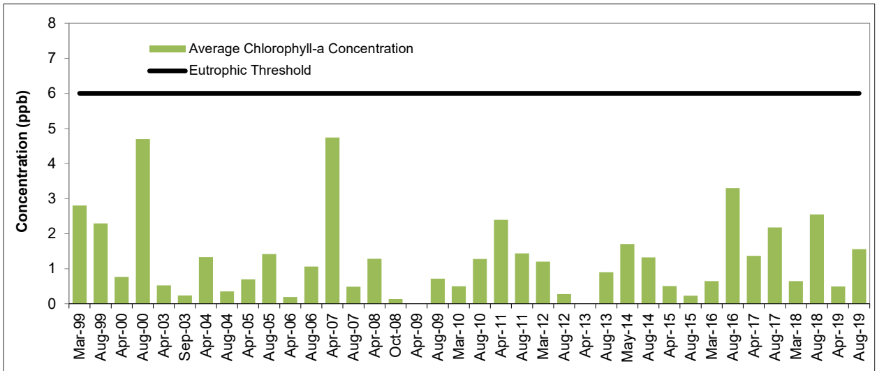
Figure 8. Average chlorophyll-a concentrations, 1999-2019.
