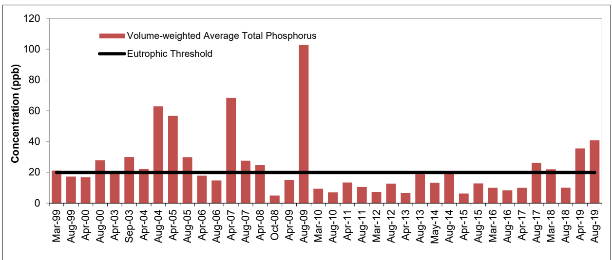
Figure 7. Volume-weighted average total phosphorus concentrations, 1999-2019.
