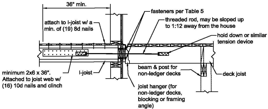
Figure 17A. Lateral Load Device with Joists Perpendicular to Deck Joists
