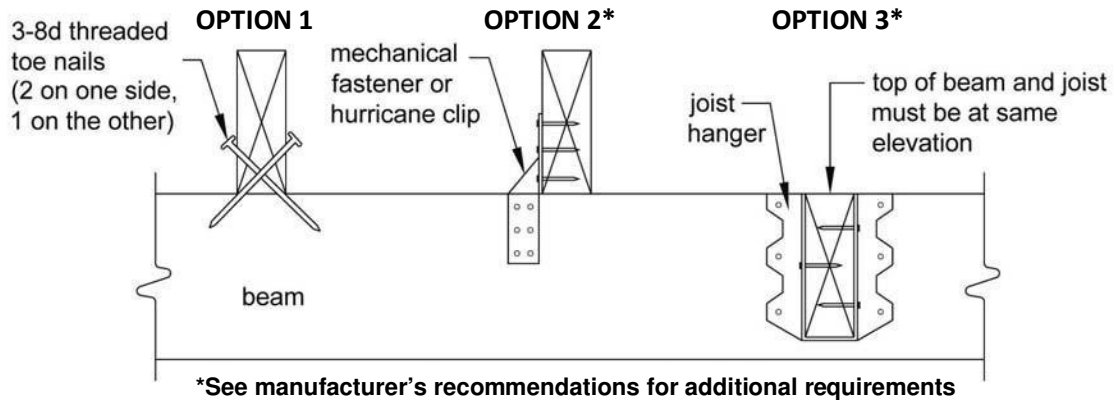
Figure 5. Joist-to-Beam Detail
