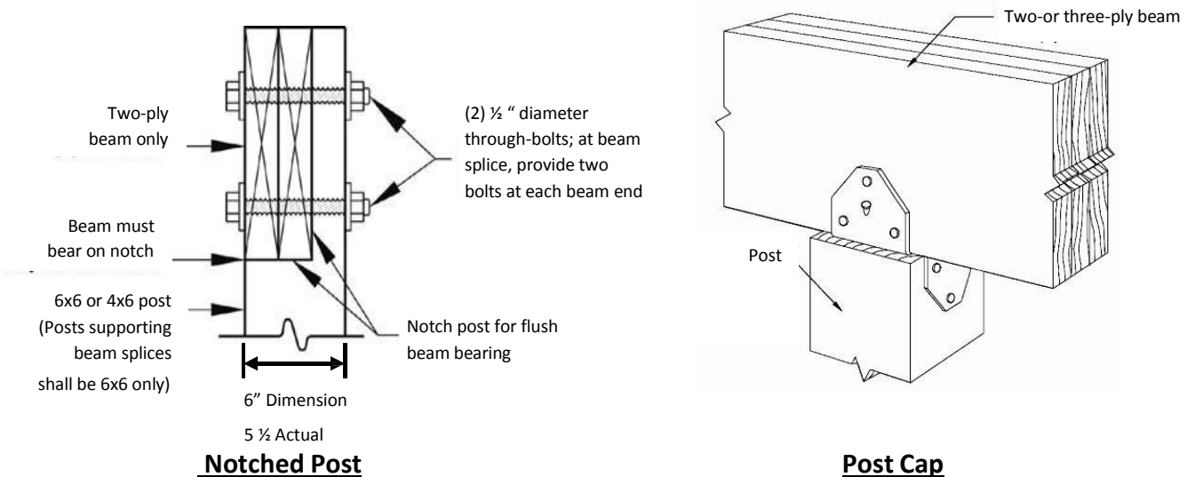
Figure 7. Post to Beam Connection
