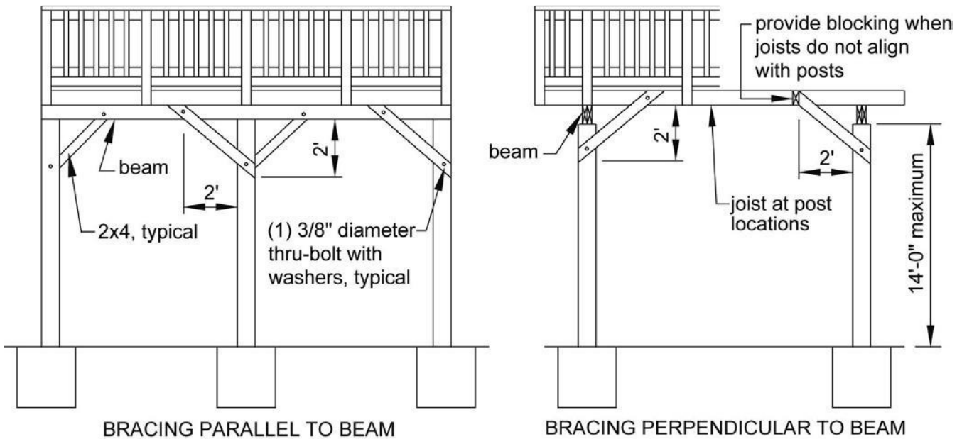
Figure 15. Diagonal Bracing Requirements
