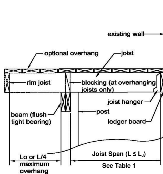
Figure 2A. Joist Span – Joist Attached at House and Bearing over
